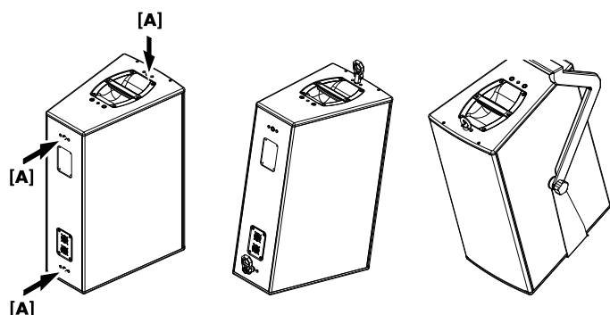
V7P loudspeaker
