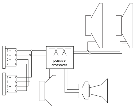
Connector wiring
